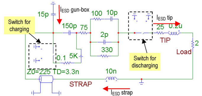
Fig. 2. SPICE equivalent circuit of a typical ESD generator.
