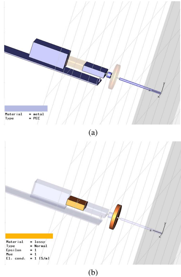
Fig. 4. Material details of the ESD simulator model in MWS. (a) Perfect electric conductive and (b) lossy dielectric regions.
